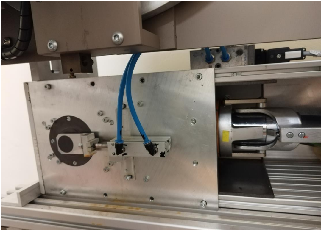
Pneumatic system
